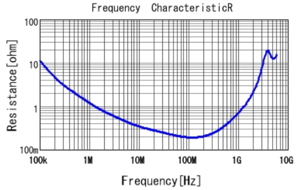
GRM21AR72E222KW01 R DCOV, 25degC
