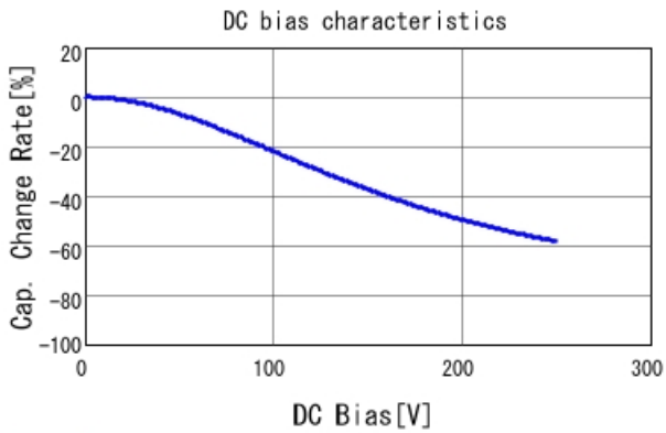
GRM21AR72E222KW01 C-DC bias capchange, 25.0degC, A
