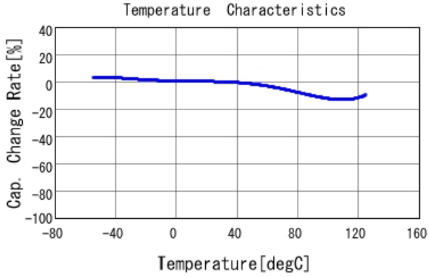
GRM21AR72E222KW01 C-Temp. capchange, DCOV, AC1Vrms
