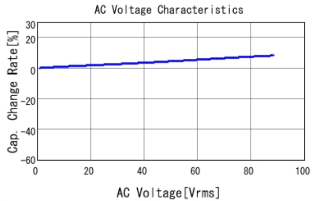
GRM21AR72E222KW01 C-AC Voltage capchange, DCOV, 25
