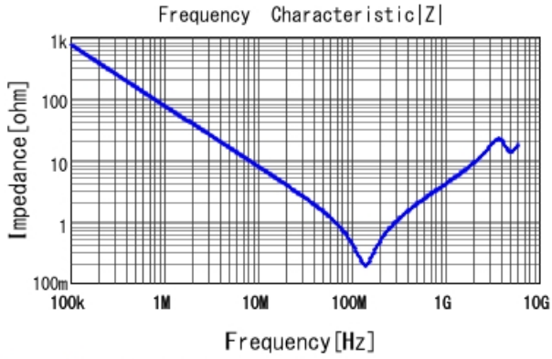
GRM21AR72E222KW01 |Z| DCOV, 25degC
