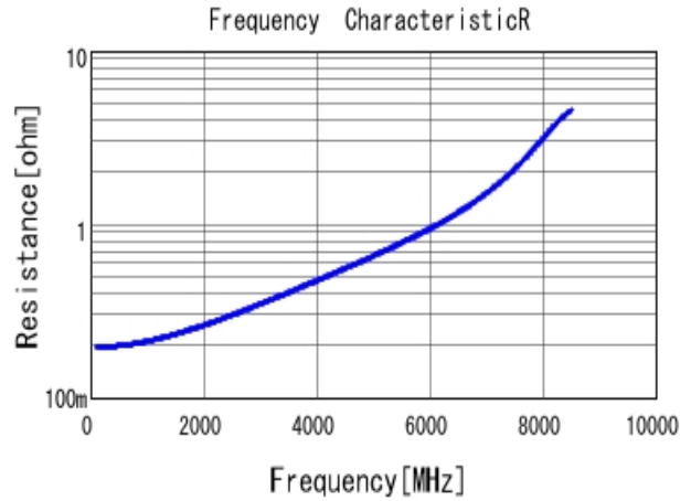
■ GRM0335C1E6R8CA01 R DCOV, 25degC
