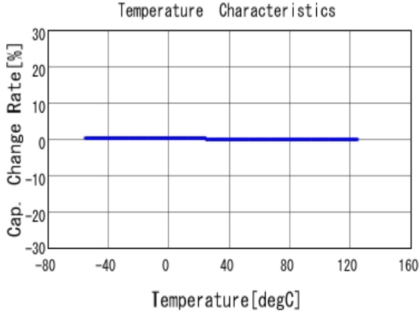
■ GRM0335C1E6R8CA01 C-Temp. capchange, DCOV, AC1Vrms
