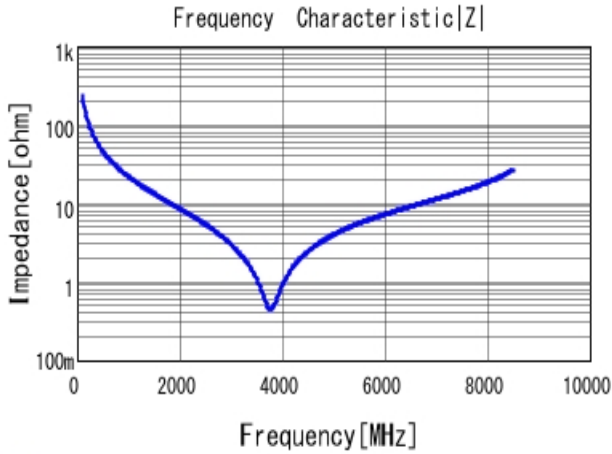
■ GRM0335C1E6R8CA01 |Z| DCOV, 25degC
