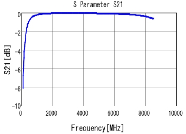
■ GRM0335C1E6R8CA01 S21 DCOV, 25degC
