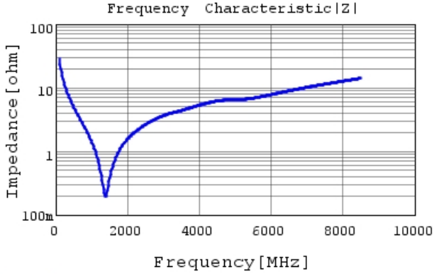
GRM0335C1E560JA01 |Z| DC0V, 25degC
