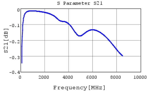
GRM0335C1E560JA01 S21 DCOV, 25degC
