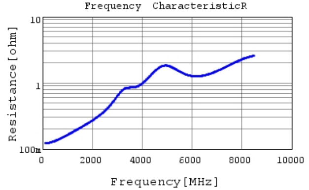
GRM0335C1E560JA01 R DC0V, 25degC
