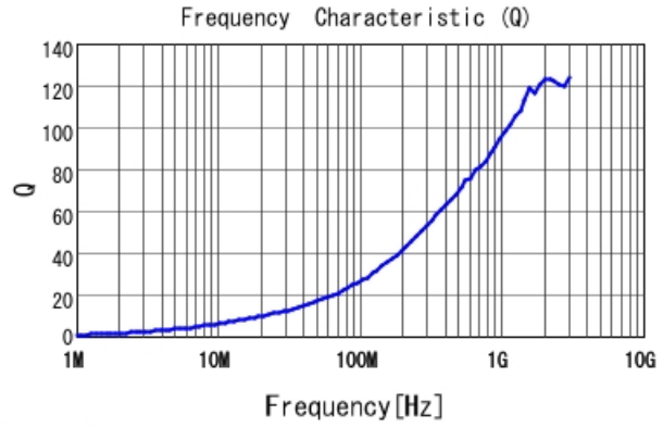
LQW15AN4N1G80 Q
