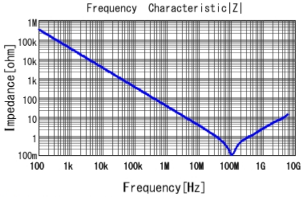
GCD188R72A472KA01 |Z| DCOV, 25degC
