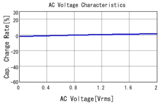
GCD188R72A472KA01 C-AC Voltage capchange, DCOV, 25.0d
