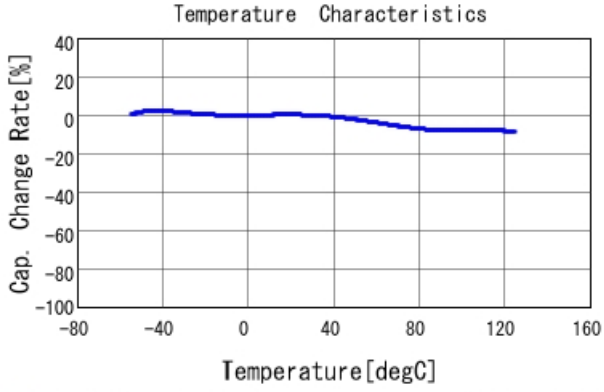
■ GCD188R72A472KA01 C-Temp. capchange, DCO. 0V, AC1. 0Vrm
