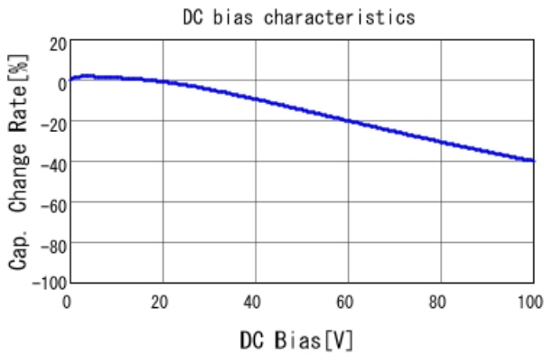
GCD188R72A472KA01 C-DC bias capchange, 25.0degC, AC1.
