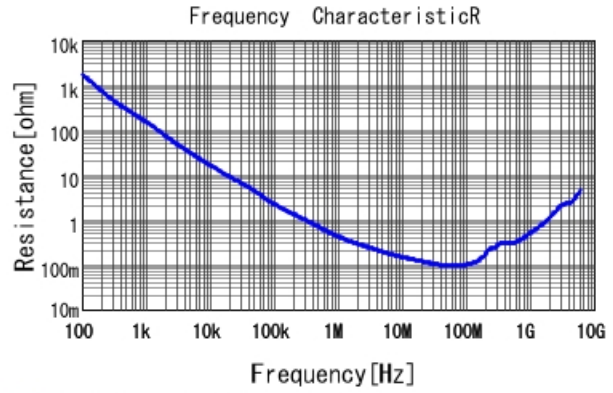
GCD188R72A472KA01 R DCOV, 25degC
