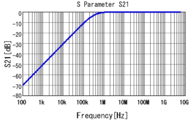
■ GCD188R72A472KA01 S21 DCOV, 25degC
