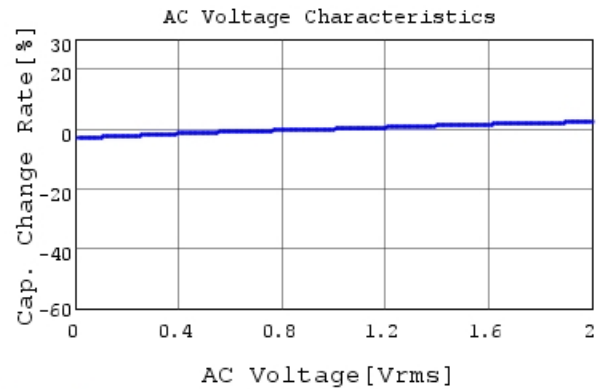
GRM033B11E221KA01 C-AC Voltage capchange, Dc
