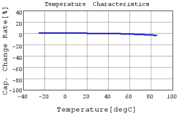
GRM033B11E221KA01 C-Temp. capchange, DC0.0V,
