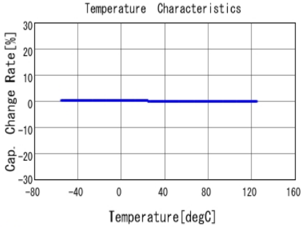
■ GRM0335C1E2R7CA01 C-Temp. capchange, DCOV, AC1Vrms
