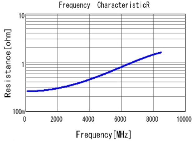
■ GRM0335C1E2R7CA01 R DC0V, 25degC
