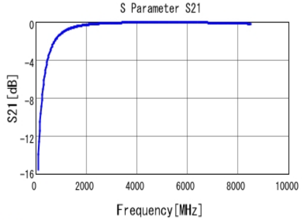
■ GRM0335C1E2R7CA01 S21 DCOV, 25degC
