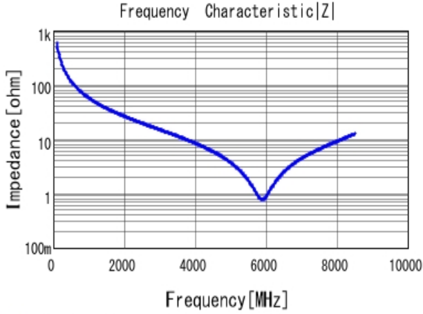
■ GRM0335C1E2R7CA01 |Z| DC0V, 25degC
