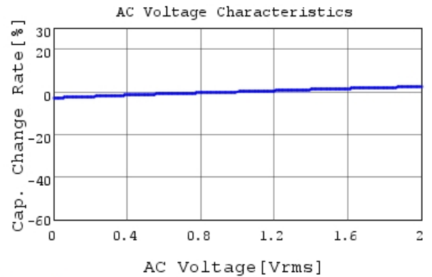
RDER71H104K0S1H03A C-AC Voltage capchange, I
