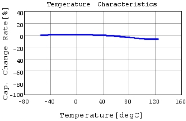
RDER71H104K0S1H03A C-Temp. capchange, DC0.0V
