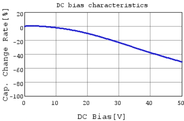
RDER71H104K0S1H03A C-DC bias capchange, 25.0
