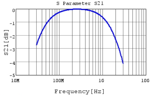
RDE5C1H560J0M1H03A S21 DCOV, 25degC
