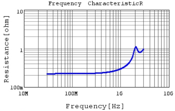
RDE5C1H560J0M1H03A R DCOV, 25degC
