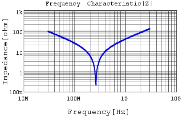
RDE5C1H560J0M1H03A |Z| DCOV, 25degC
