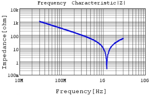
RCE5C1H5R0C0DBH03A |Z| DC0V, 25degC
