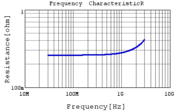
RCE5C1H5R0C0DBH03A R DC0V, 25degC
