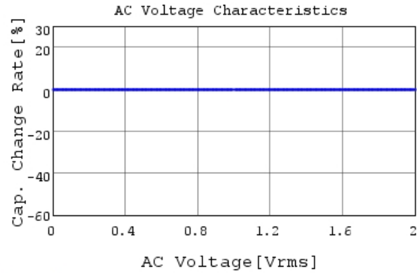
RCE5C1H5R0C0DBH03A C-AC Voltage capchange, I
