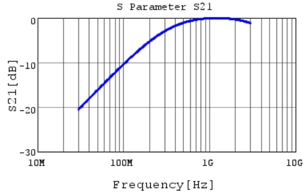
RCE5C1H5R0C0DBH03A S21 DC0V, 25degC
