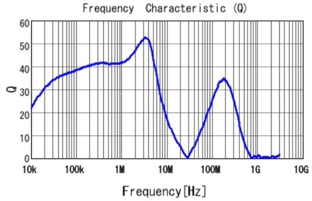
1217AS-H-8R2M Q
