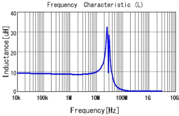
1217AS-H-8R2M L
