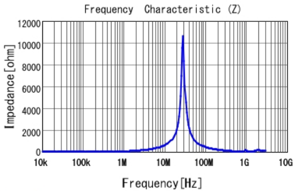
1217AS-H-8R2M |Z|
