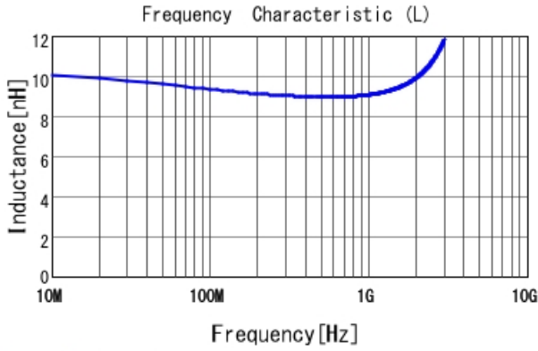
LQP03TQ9N1H02 L
