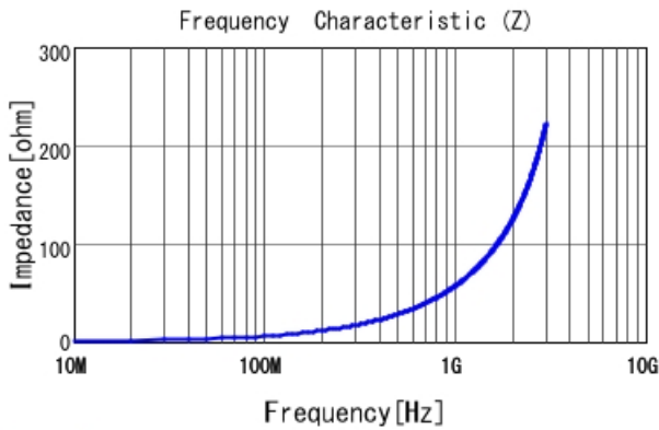
LQP03TQ9N1H02 |Z|
