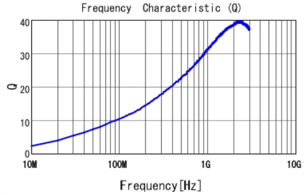
LQP03TQ9N1H02 Q
