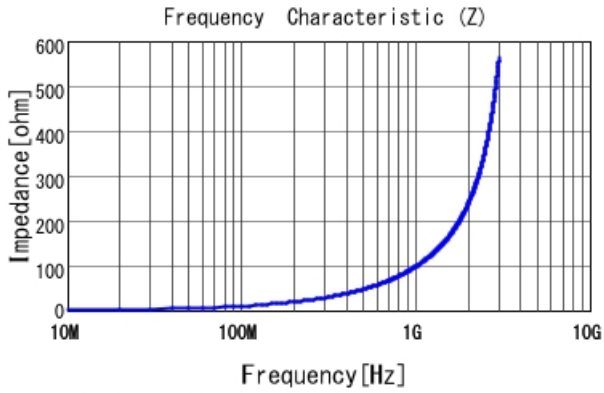
LQP15MN15NG02 |Z|
