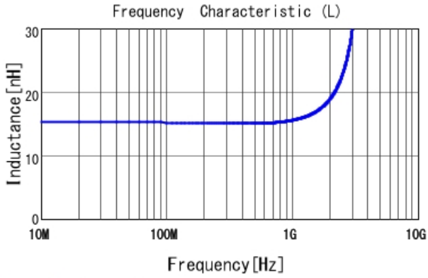
LQP15MN15NG02 L
