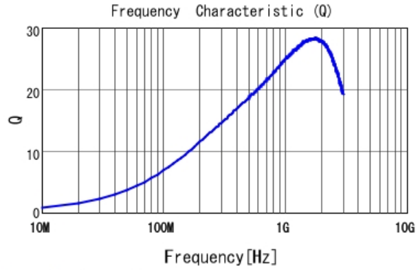
LQP15MN15NG02 Q
