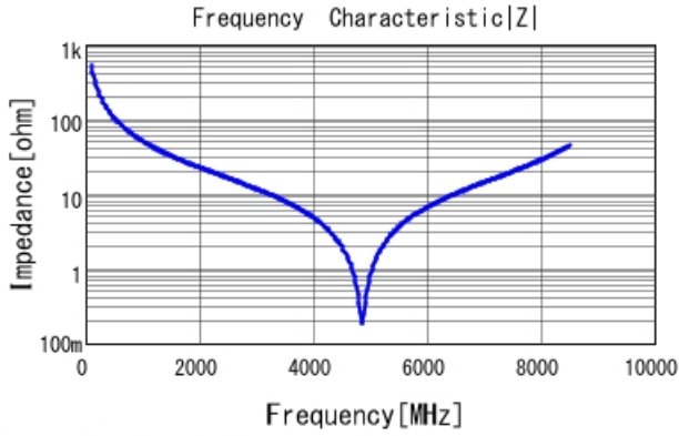
GQM1875C2E3R0BB12 |Z| DCOV, 25degC
