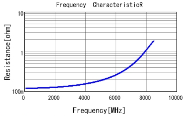
GQM1875C2E3R0BB12 R DCOV, 25degC
