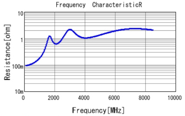
GRM2162C2A151JA01 R DCOV, 20degC
