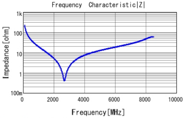
GRM1885C1H7R0DA01 |Z| DCOV, 25degC
