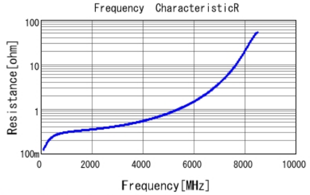
GRM1885C1H7R0DA01 R DCOV, 25degC
