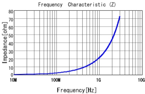
LQP03TG3N4B02 |Z|
