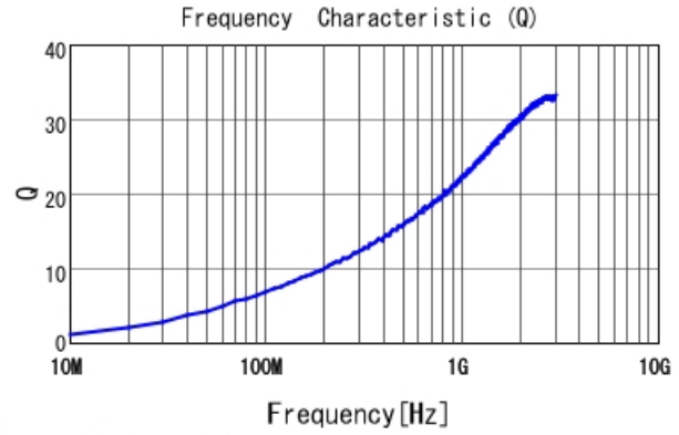
LQP03TG3N4B02 Q
