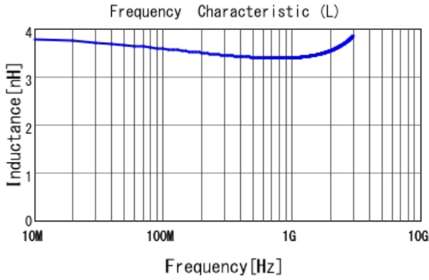
LQP03TG3N4B02 L
