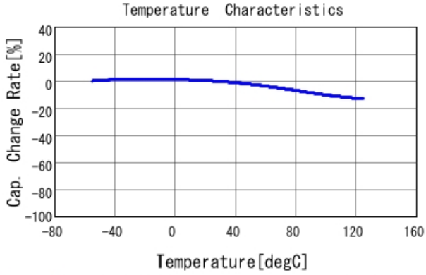
GRM31MR71E225KA93 C-Temp. capchange, DC0.0V, AC1.C
