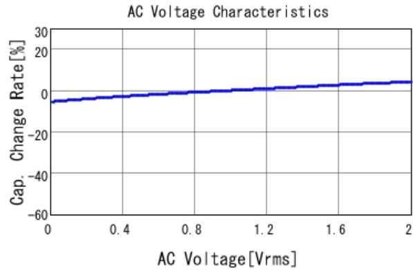
GRM31MR71E225KA93 C-AC Voltage capchange, DCOV, 25
