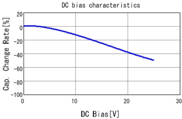
GRM31MR71E225KA93 C-DC bias capchange, 25.0degC, A
