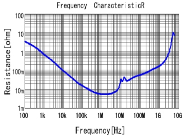
■ GRM31MR71E105KA01 R DCOV, 25degC
