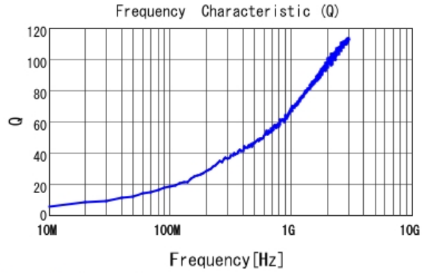
LQP03HQ1N2C02 Q
