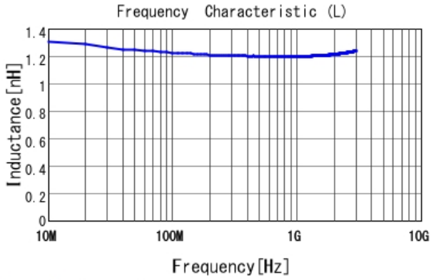
LQP03HQ1N2C02 L
