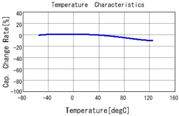
GRM31CR71H225KA88 C-Temp. capchange, DC0.0V, AC1.C
