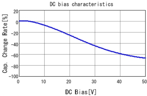
GRM31CR71H225KA88 C-DC bias capchange, 25.0degC, A
