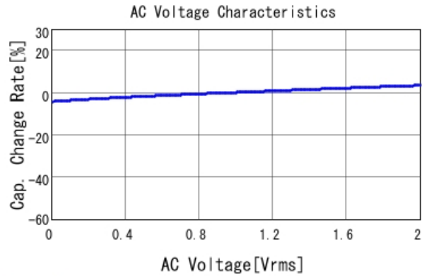
GRM31CR71H225KA88 C-AC Voltage capchange, DCOV, 25
