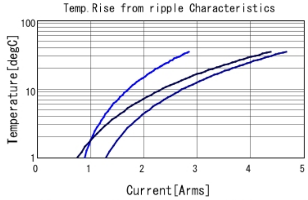
GRM31CR71H225KA88 Temp. rise — 100kHz — 500
