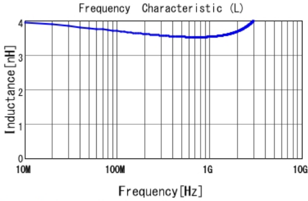
LQP03TN3N5B02 L
