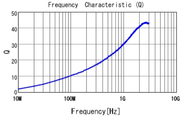
LQP03TN3N5B02 Q
