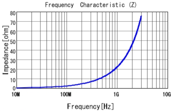
LQP03TN3N5B02 |Z|
