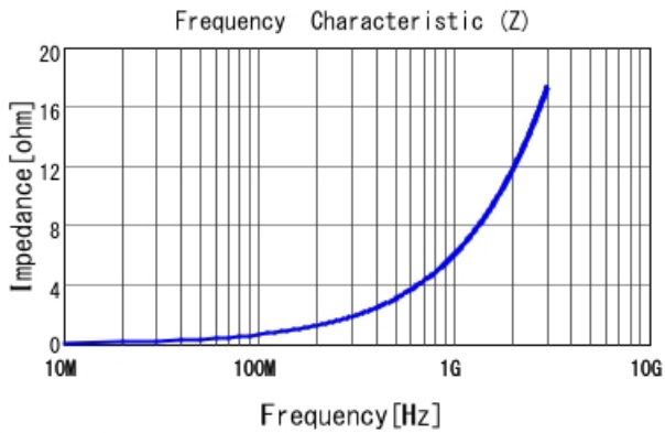
LQP02TQ1N0B02 |Z|
