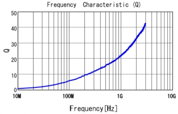
LQP02TQ1N0B02 Q
