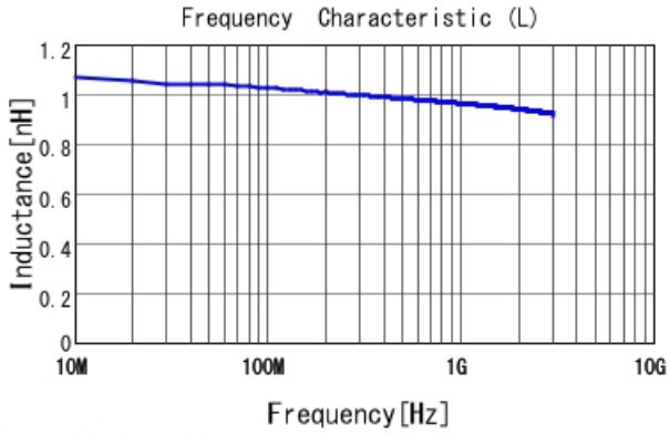
LQP02TQ1N0B02 L
