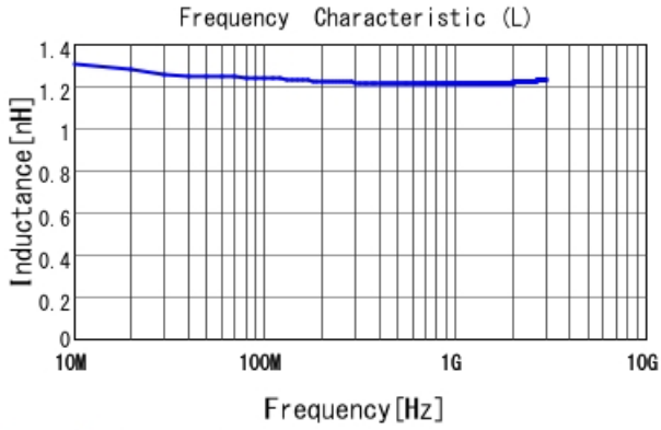
LQP03TQ1N2B02 L
