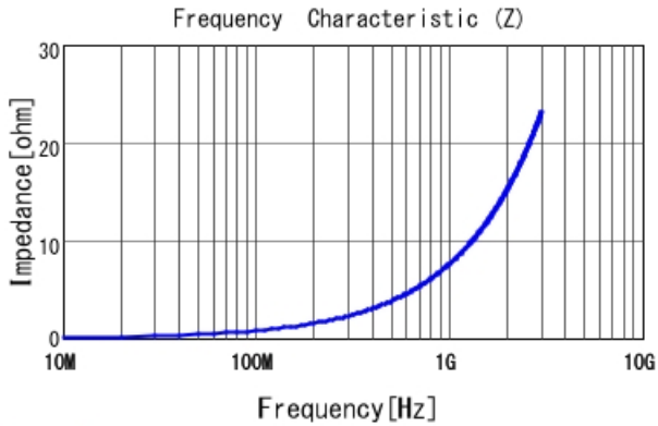
LQP03TQ1N2B02 |Z|
