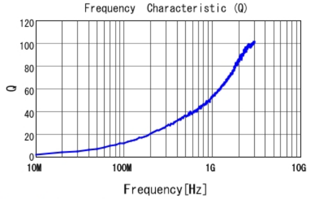
LQP03TQ1N2B02 Q
