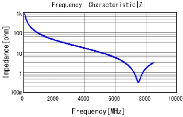
GJM0335C1E1R8WB01 |Z| DCOV, 25degC
