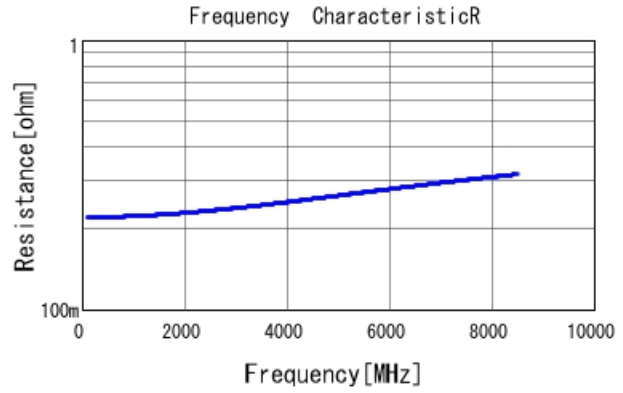
GJM0335C1E1R8WB01 R DCOV, 25degC
