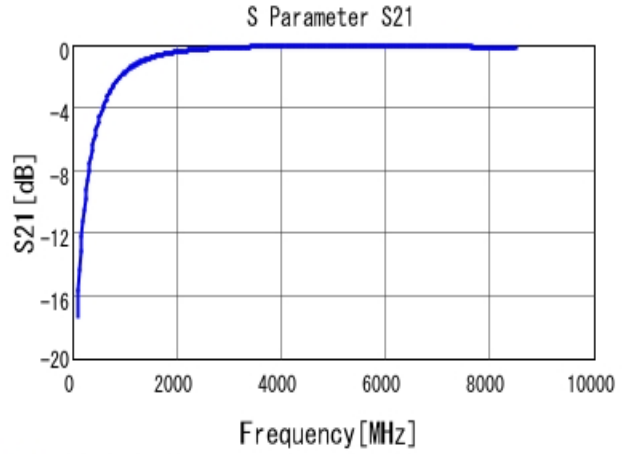
■ GRM1555C1H2R2CA01 S21 DCOV, 25degC
