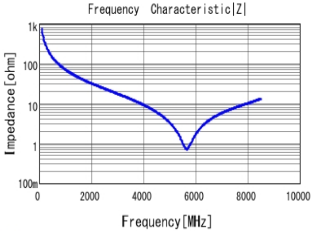
■ GRM1555C1H2R2CA01 |Z| DC0V, 25degC
