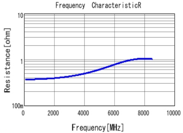
■ GRM1555C1H2R2CA01 R DC0V, 25degC
