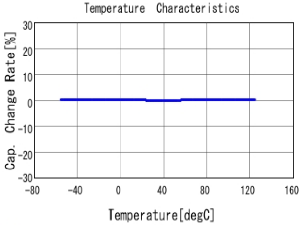
■ GRM1555C1H2R2CA01 C-Temp. capchange, DCOV, AC1Vrms
