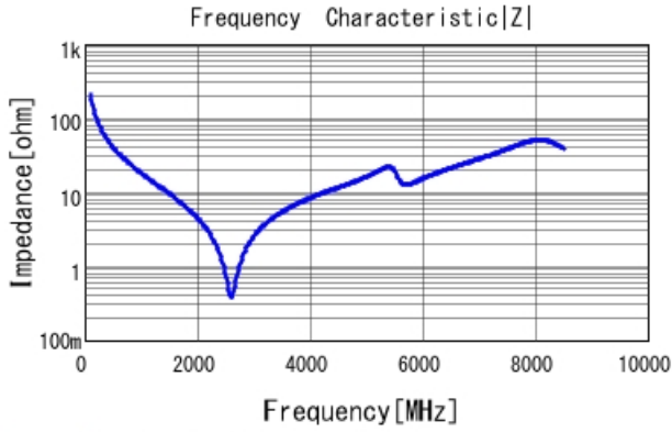
GRM1885C1H7R5DA01 |Z| DCOV, 25degC
