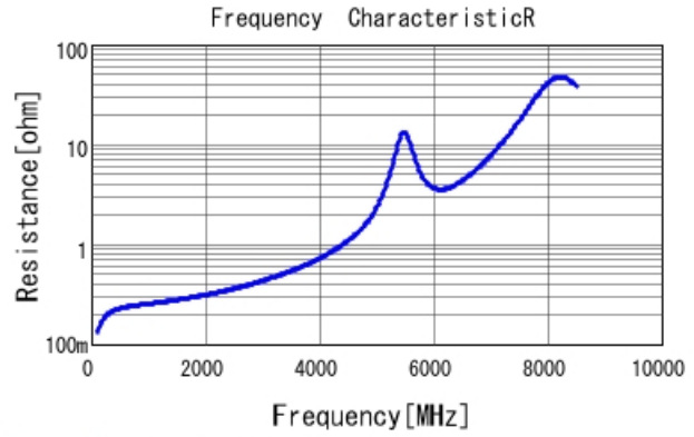
GRM1885C1H7R5DA01 R DCOV, 25degC
