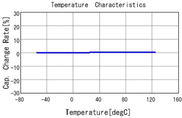
GRM1885C1H7R5DA01 C-Temp. capchange, DC0V, AC1Vrms
