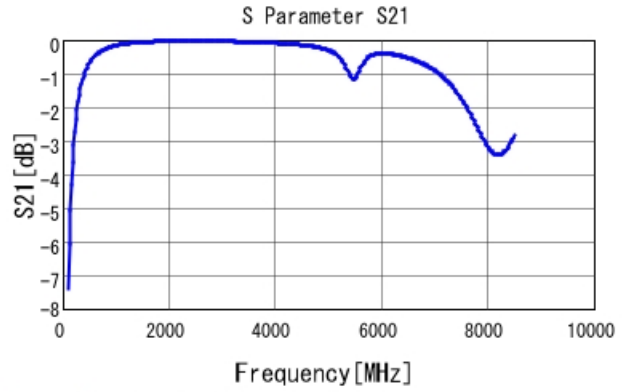
GRM1885C1H7R5DA01 S21 DC0V, 25degC
