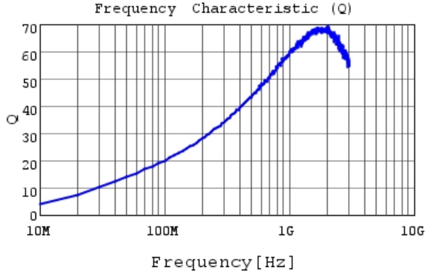
LQW15AN27NG00 Q
