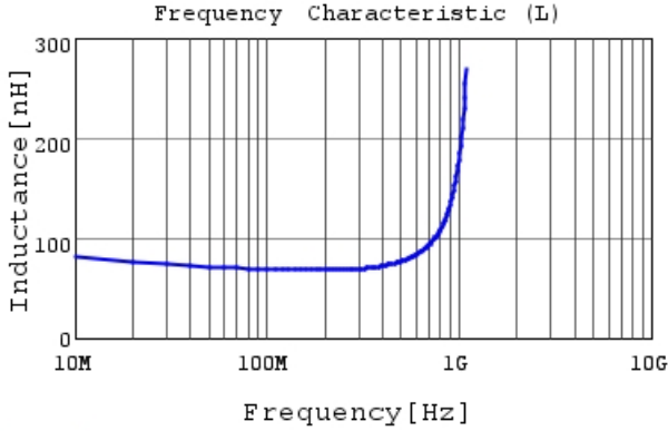
LQG15HN68NJ02 L
