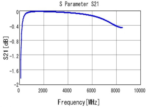
■ GRM0332C1H220JA01 S21 DCOV, 20degC
