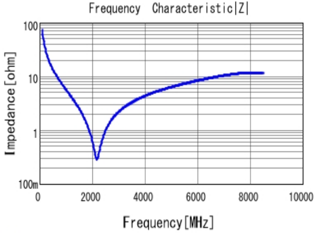
■ GRM0332C1H220JA01 |Z| DCOV, 20degC
