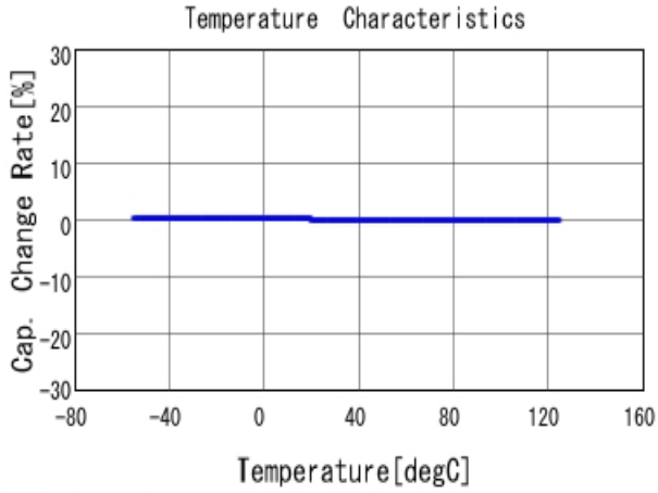
■ GRM0332C1H220JA01 C-Temp. capchange, DCOV, AC1Vrms
