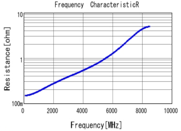
■ GRM0332C1H220JA01 R DCOV, 20degC
