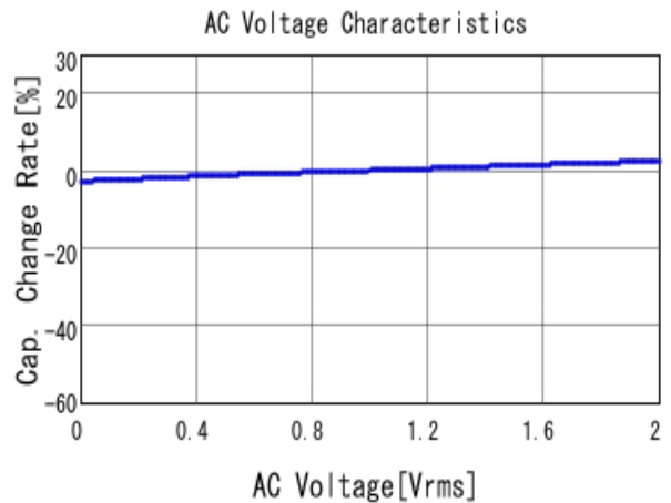
■ RCER71H104K0DBH03A C-AC Voltage capchange, DC0V, 25.0
