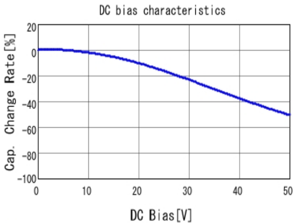
■ RCER71H104K0DBH03A C-DC bias capchange, 25.0degC, AC1
