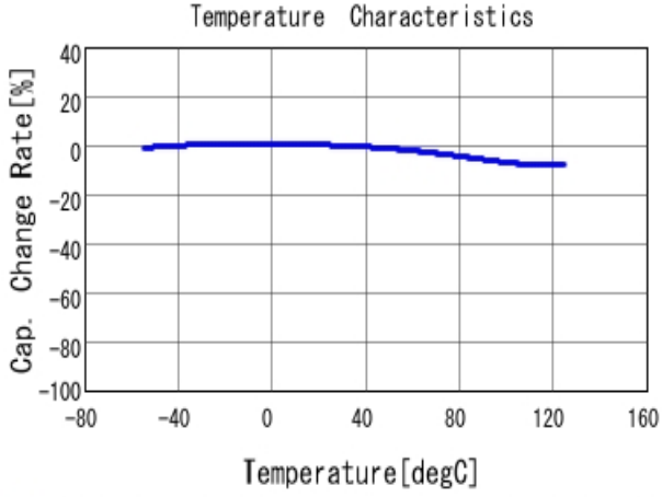
■ RCER71H104K0DBH03A C-Temp. capchange, DC0.0V, AC1.0Vr
