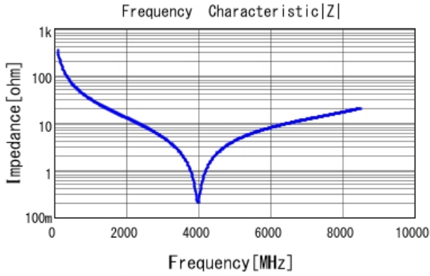
GJM1555C1H4R7CB01 |Z| DCOV, 25degC
