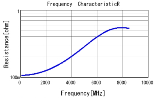
GJM1555C1H4R7CB01 R DCOV, 25degC
