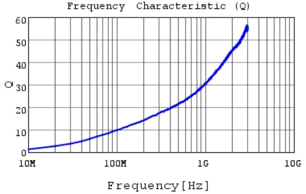
LQP02HQ3N7B02 Q
