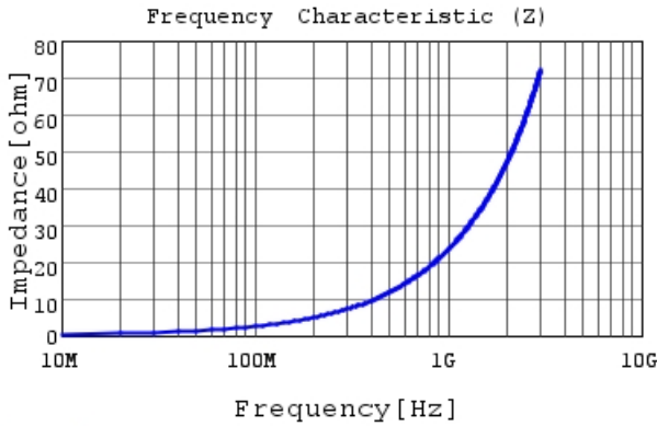
LQP02HQ3N7B02 |Z|
