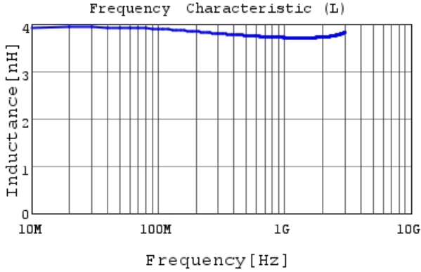
LQP02HQ3N7B02 L
