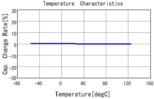
GCM2165C2A681JA16 C-Temp. capchange, DCOV, AC1Vrms
