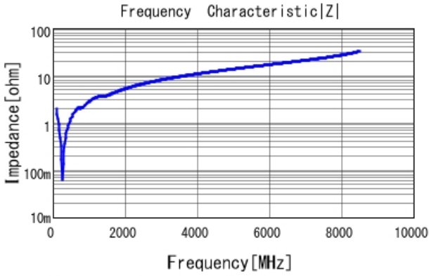
GCM2165C2A681JA16 |Z| DCOV, 25degC
