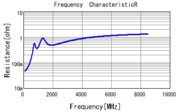
GCM2165C2A681JA16 R DCOV, 25degC
