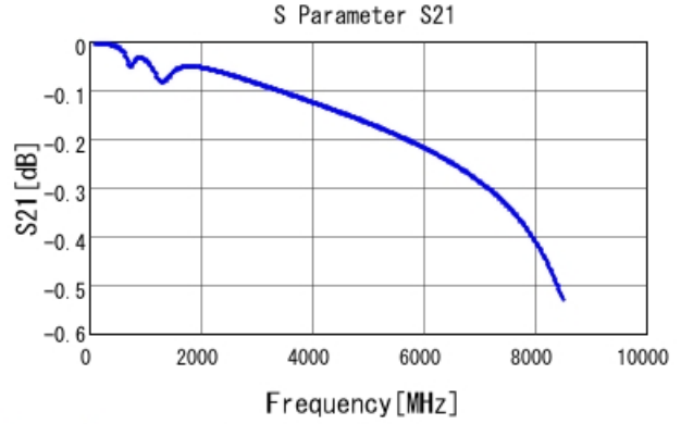
GCM2165C2A681JA16 S21 DCOV, 25degC
