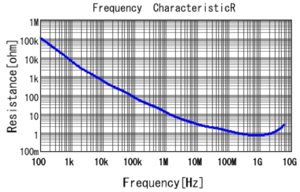
GRM033R71C151KA01 R DCOV, 25degC
