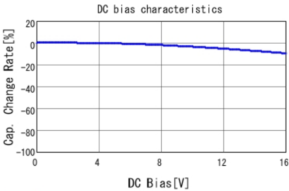
GRM033R71C151KA01 C-DC bias capchange, 25.0degC, A
