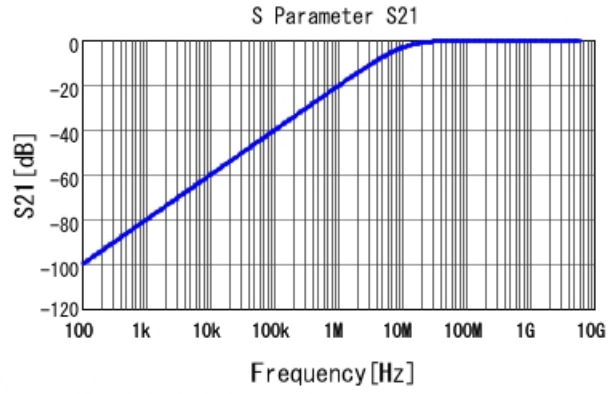
GRM033R71C151KA01 S21 DC0V, 25degC
