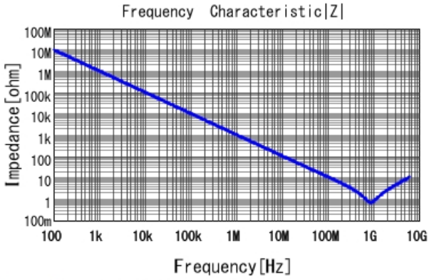
GRM033R71C151KA01 |Z| DCOV, 25degC
