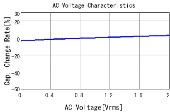
GRM033R71C151KA01 C-AC Voltage capchange, DCOV, 25
