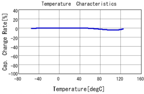
GRM033R71C151KA01 C-Temp. capchange, DC0.0V, AC1.C
