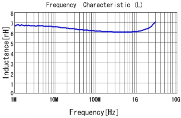
LQW15AN6N2B8Z L
