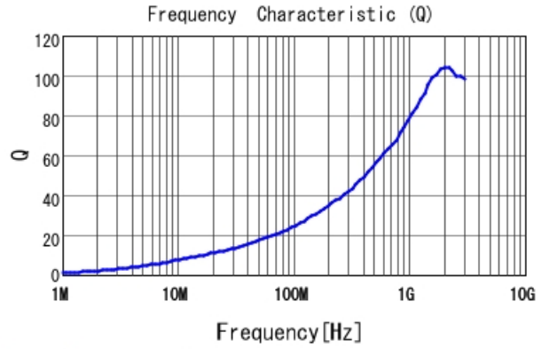
LQW15AN6N2B8Z Q
