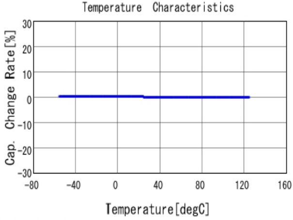
■ GRM1885C1H330JA01 C-Temp. capchange, DCOV, AC1Vrms
