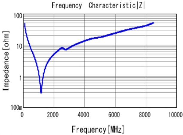
■ GRM1885C1H330JA01 |Z| DCOV, 25degC
