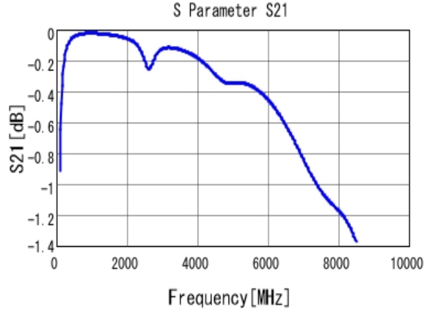
■ GRM1885C1H330JA01 S21 DCOV, 25degC
