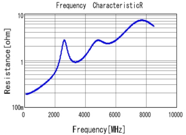
■ GRM1885C1H330JA01 R DCOV, 25degC
