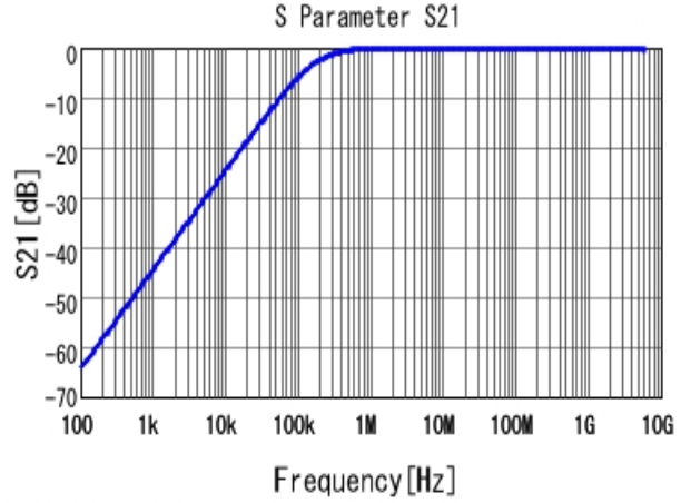
■ GRM155R71C103KA01 S21 DCOV, 25degC
