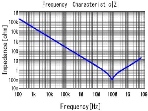
■ GRM155R71C103KA01 |Z| DCOV, 25degC
