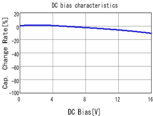
■ GRM155R71C103KA01 C-DC bias capchange, 25.0degC, AC1.
