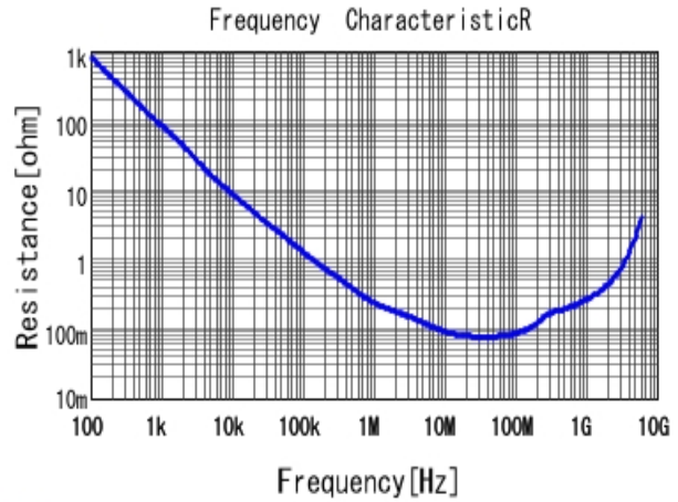
■ GRM155R71C103KA01 R DCOV, 25degC
