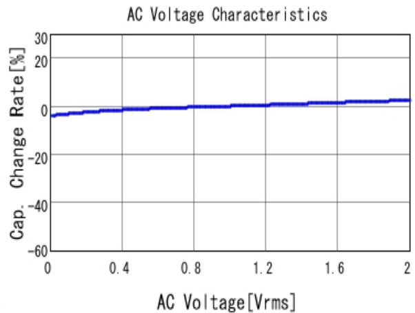
■ GRM155R71C103KA01 C-AC Voltage capchange, DCOV, 25.0d
