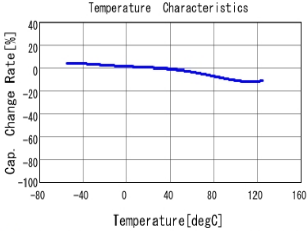
■ GRM155R71C103KA01 C-Temp. capchange, DCO. 0V, AC1.0V rm
