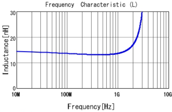
LQP03TN13NH02 L
