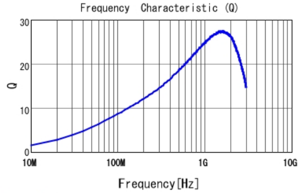
LQP03TN13NH02 Q
