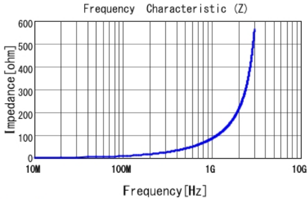
LQP03TN13NH02 |Z|
