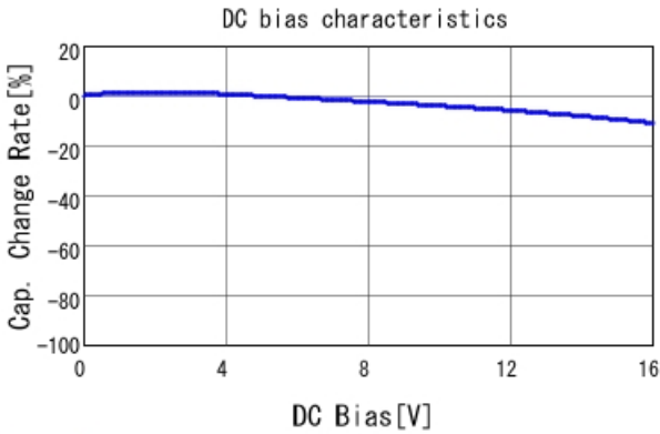
GRM155R61C103KA01 C-DC bias capchange, 25.0degC, A
