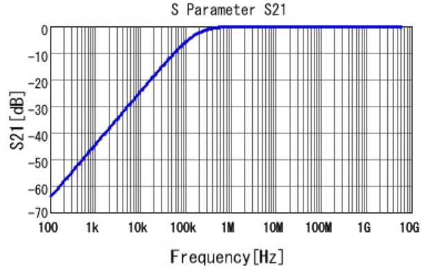
GRM155R61C103KA01 S21 DC0V, 25degC
