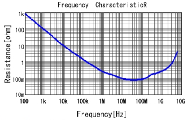
GRM155R61C103KA01 R DCOV, 25degC
