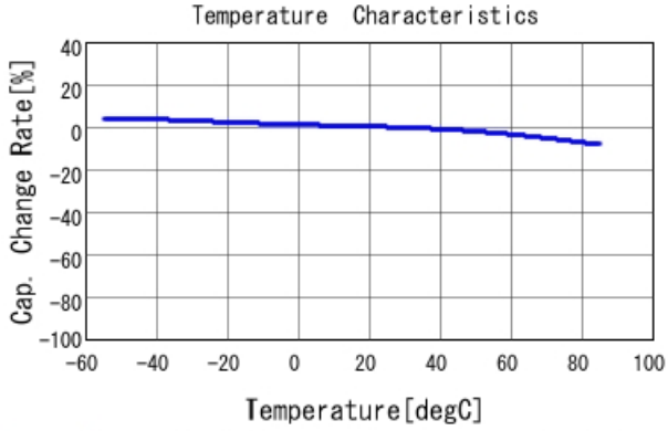
GRM155R61C103KA01 C-Temp. capchange, DC0.0V, AC1.C
