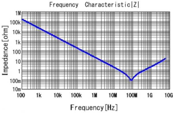
GRM155R61C103KA01 |Z| DCOV, 25degC
