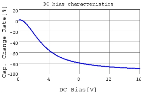
GRM033R61C224KE14 C-DC bias capchange, 25.0c
