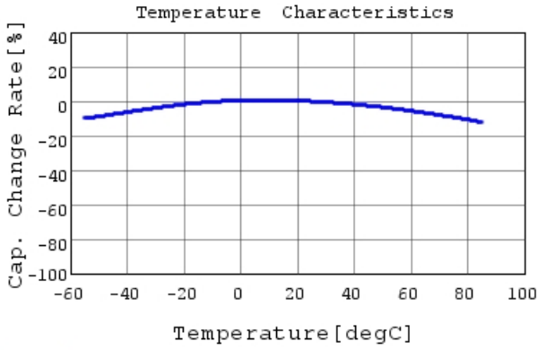
GRM033R61C224KE14 C-Temp. capchange, DC0.0V,
