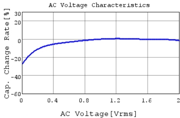
GRM033R61C224KE14 C-AC Voltage capchange, Dc
