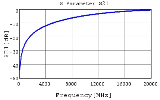
GCQ1555C1HR10BB01 S21 DCOV, 25degC
