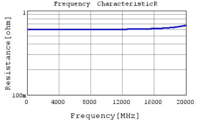
GCQ1555C1HR10BB01 R DC0V, 25degC
