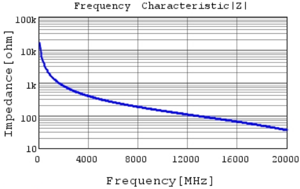
GCQ1555C1HR10BB01 |Z| DC0V, 25degC
