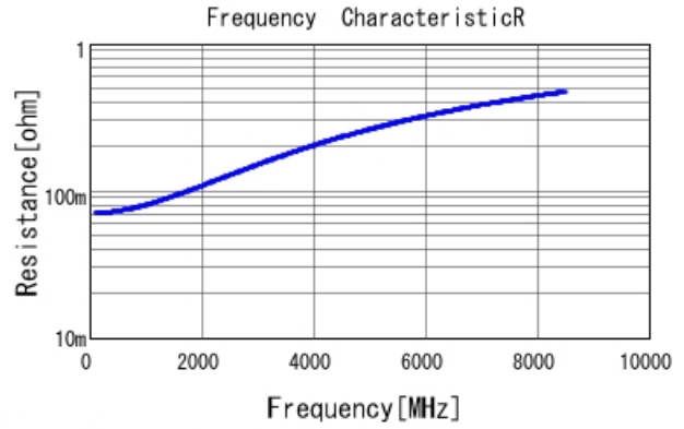
GJM0335C1E5R7CB01 R DCOV, 25degC
