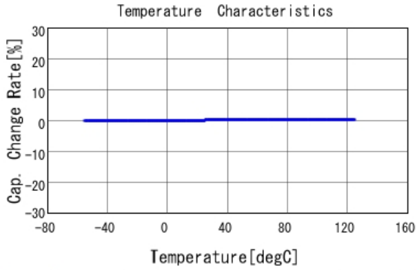
GJM0335C1E5R7CB01 C-Temp. capchange, DC0V, AC1Vrms
