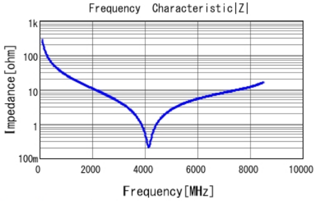
GJM0335C1E5R7CB01 |Z| DCOV, 25degC
