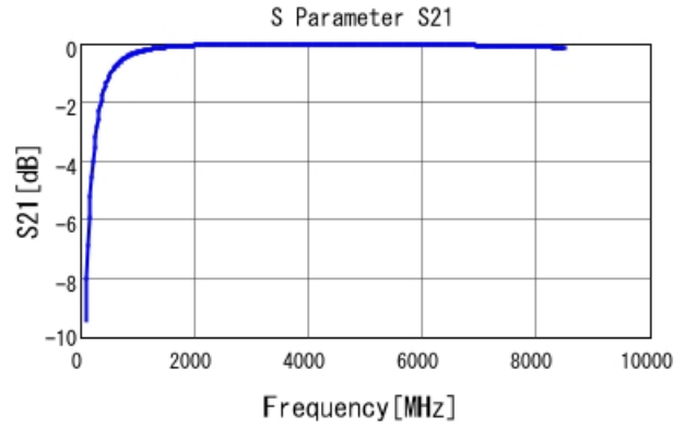
GJM0335C1E5R7CB01 S21 DC0V, 25degC
