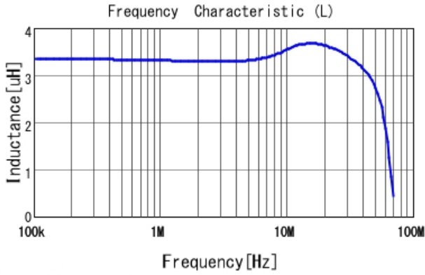
LQM21PZ3R3MG0 L
