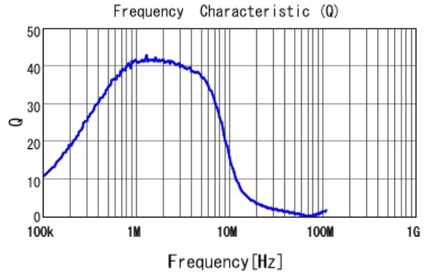
LQM21PZ3R3MG0 Q
