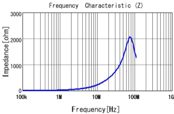
LQM21PZ3R3MG0 |Z|
