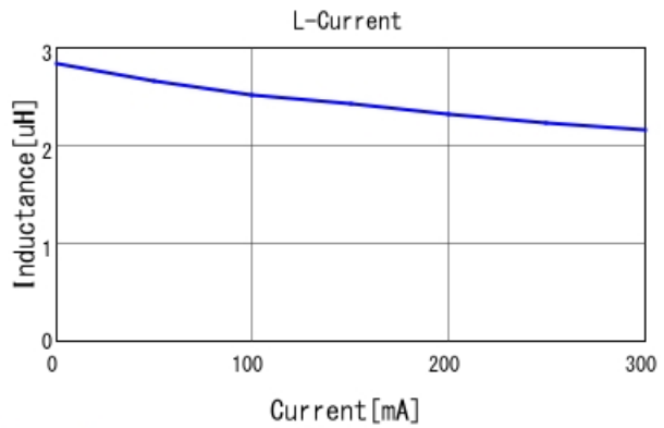
LQM21PZ3R3MG0 L-Current 20degC
