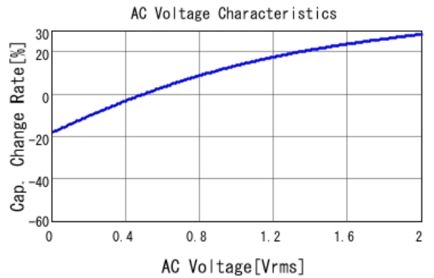
GRM32ER61E226KE15 C-AC Voltage capchange, DCOV, 25
