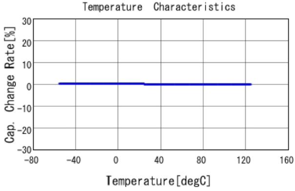
■ GCM0335C1H120FA16 C-Temp. capchange, DCOV, AC1Vrms
