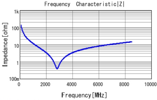
GCM0335C1H120FA16 |Z| DC0V, 25degC
