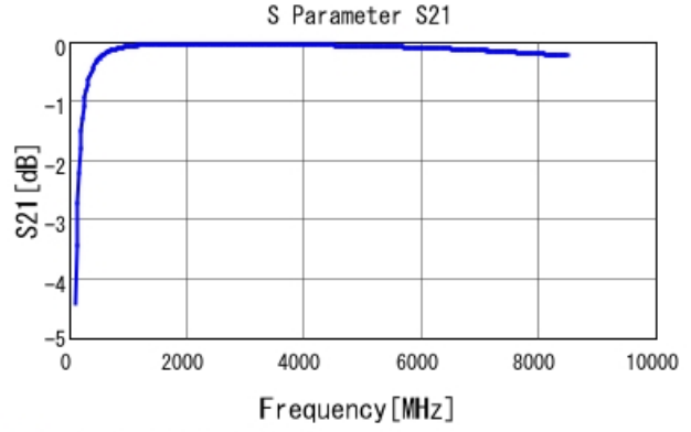
■ GCM0335C1H120FA16 S21 DCOV, 25degC
