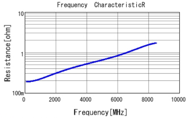
GCM0335C1H120FA16 R DC0V, 25degC
