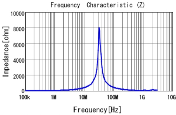
1273AS-H-6R8N |Z|
