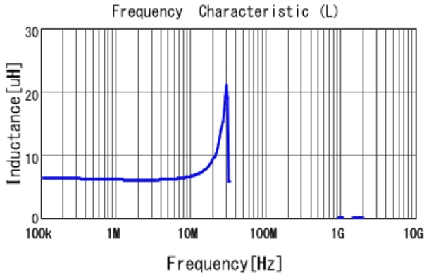
1273AS-H-6R8N L
