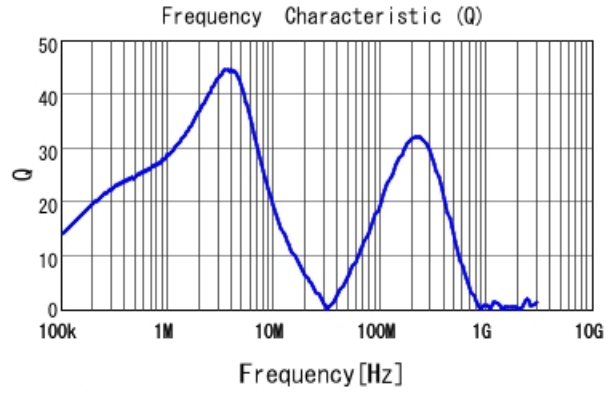
1273AS-H-6R8N Q
