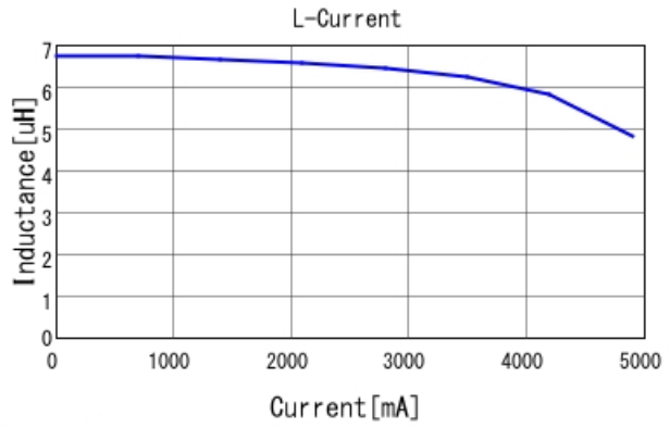
1273AS-H-6R8N L-Current 20degC
