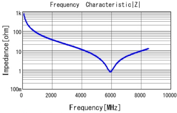
GRM1555C1H2R0BA01 |Z| DCOV, 25degC
