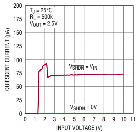
LT3065-2.5 Quiescent Current
