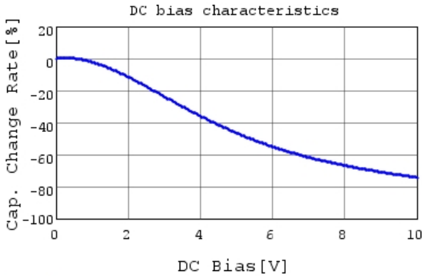
GRM155Z71A225KE44 C-DC bias capchange, 25.0c
