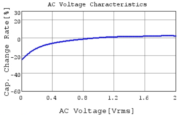
GRM155Z71A225KE44 C-AC Voltage capchange, Dc
